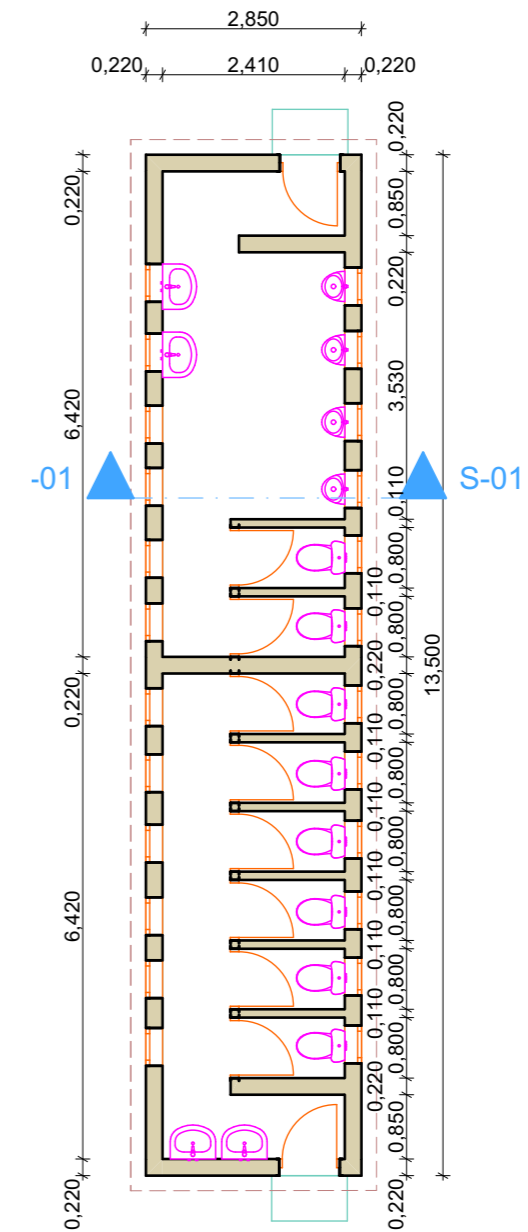
FLOOR PLAN
