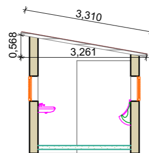
SECTION PLAN
