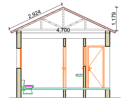
SECTION PLAN
